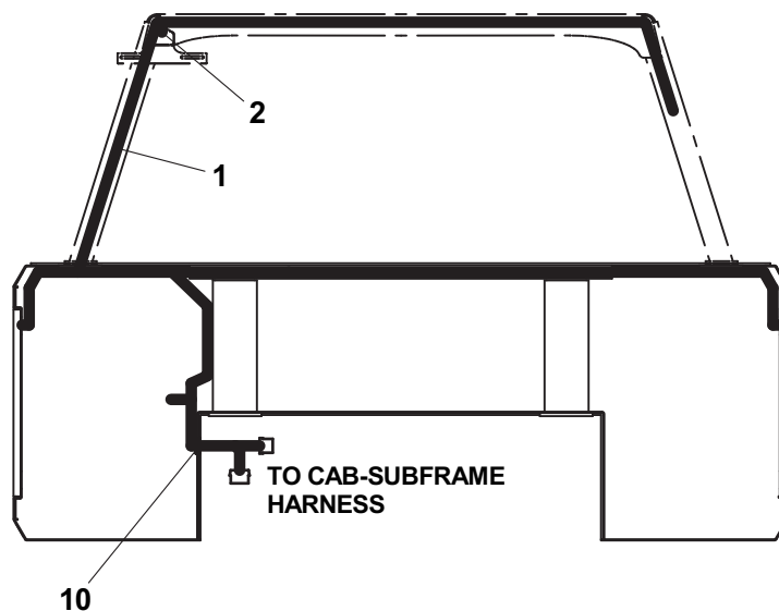
TUNNEL TOOL COMPARTMENT MOUNTED LIGHT PYLON
